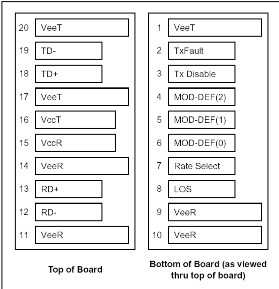
Figure 1. Pin Definitions
